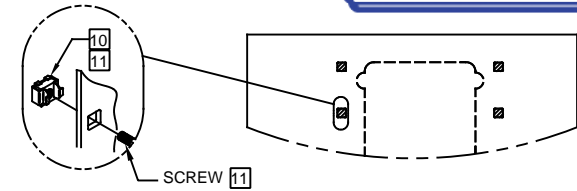
BOWL MOUNTING DETAIL
